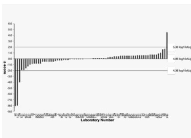
Figure 2a, histogram of z-scores in M242e13, aerobic plate count in milk powder. Apart from a few extreme results, the distribution is continuous.
