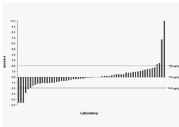
Figure 1a, symmetrical histogram of z-scores, no evidence of instability.
