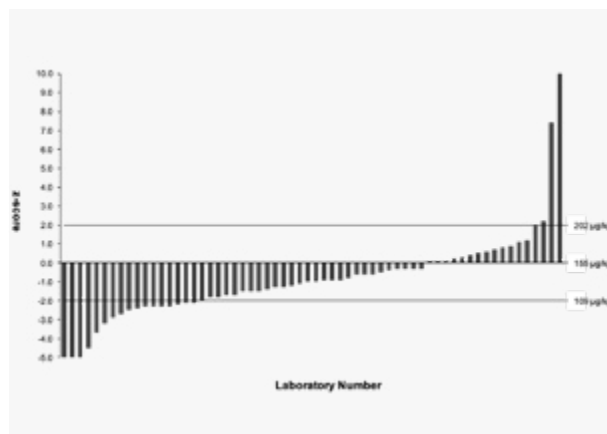
Figure 1b, skewed or asymmetrical histogram of z-scores. The direction of the skew might indicate instability.
